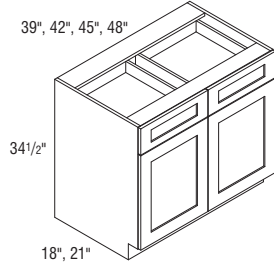
VB3934 _ _VB4834 _ _CS Center mullion
