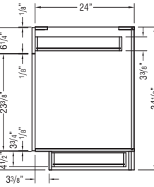
BASE CABINET with TOEKICK DRAWER
