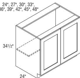
B24FH-B36FH Butt doors B39FH-B48FHCS Center mullion
