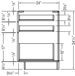
THREE-DRAWER BASE CABINET with DEEP DRAWER
