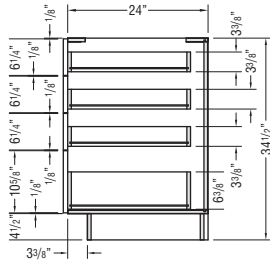
FOUR-DRAWER BASE CABINET
