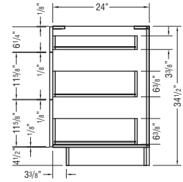
THREE-DRAWER BASE CABINET
