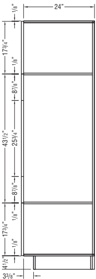
SINGLE OVEN CABINET
