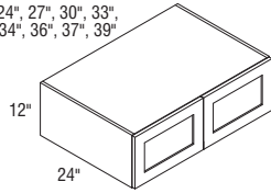
W241224-W371224 Butt doors W391224 Center mullion
