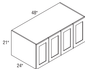
W482124 Vertical divider
