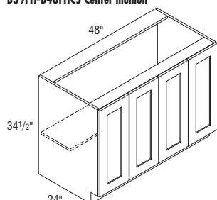
B48FH Vertical divider
