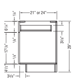
DESK BASE CABINET
