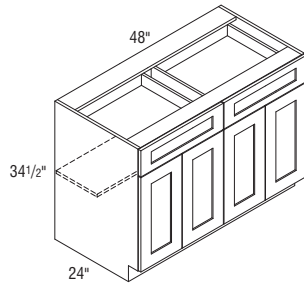
B48 Vertical divider
