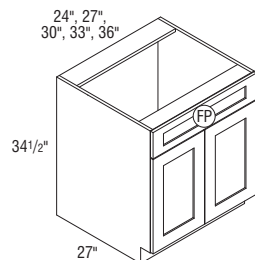
SB243427-SB363427 Butt doors
