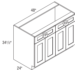
SB48 Vertical divider
