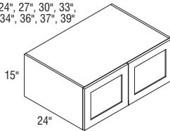
W241524-W371524 Butt doors W391524 Center mullion
