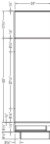
DOUBLE OVEN CABINET
