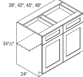
B39-B48CS Vertical divider
