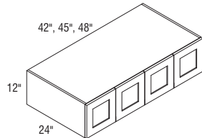
W421224-W481224 Vertical divider
