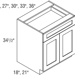
VB2434 _ _VB3634 _ _ Buttt doors
