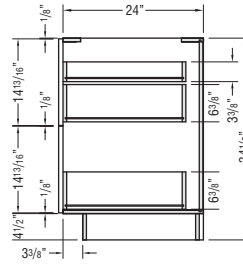
TWO-DRAWER BASE CABINET with ROLL TRAY
