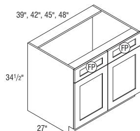
SB393427-SB483427CS Vertical divider
