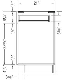
34 1/2" HIGH VANITY CABINET
