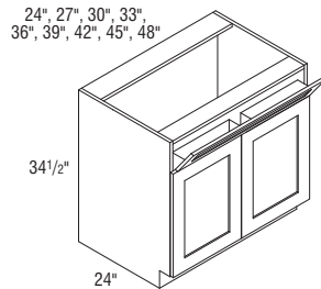
SB24ST-SB36ST Butt doors SB39ST-SB48CSST Vertical divider, two drawer fronts
