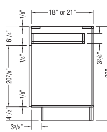
32" HIGH VANITY CABINET
