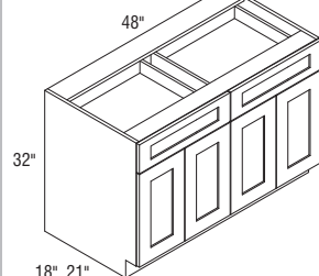
VB4832_ _ Vertical divider
