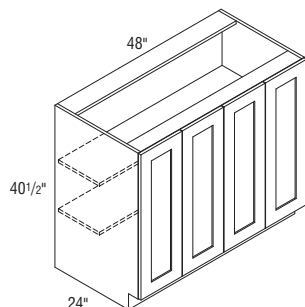
B4840FH Vertical divider
