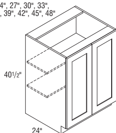
B2440FH-B3640FH Butt doors B3940FH-B4840FHCS Center mullion
