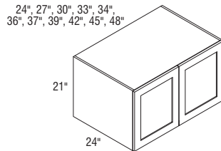
W242124-W372124 Butt doors W392124-W482124CS Center mullion
