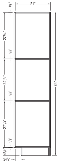
VANITY UTILITY CABINET
